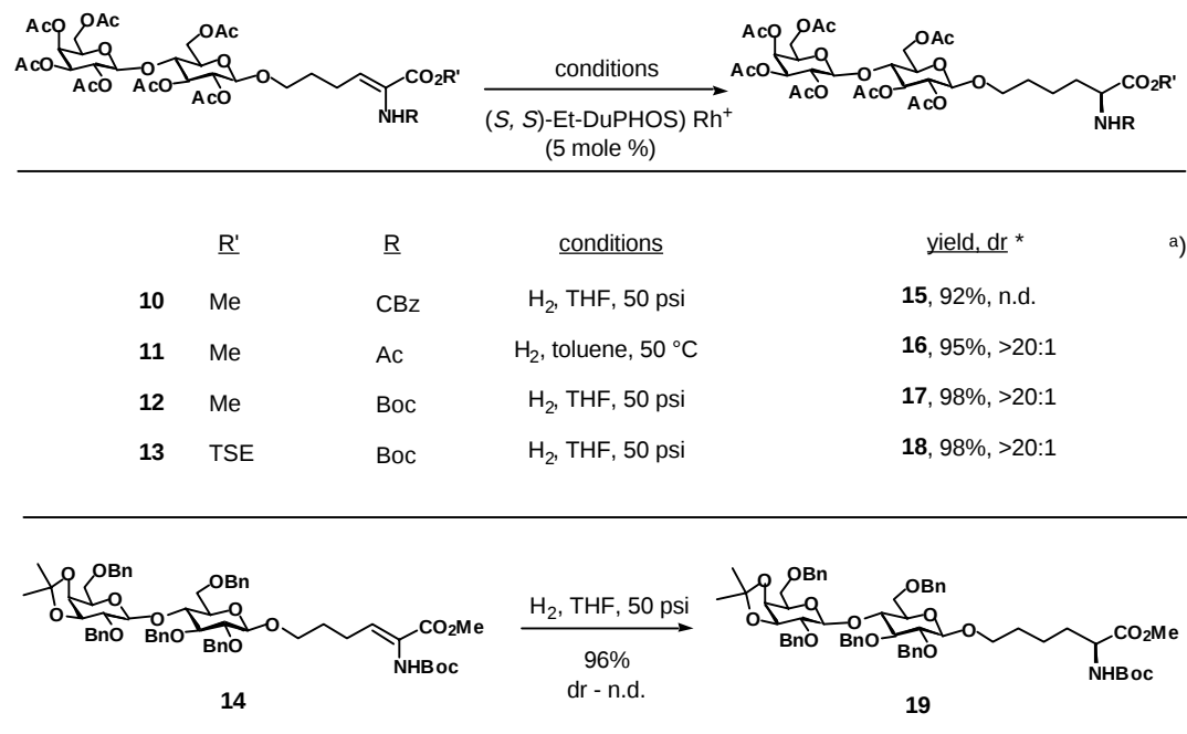
Scheme 3 Asymmetric hydrogenation reactions
