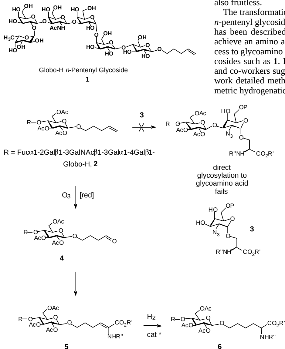
Scheme 1 Proposed synthesis of glycoamino acid derivatives
