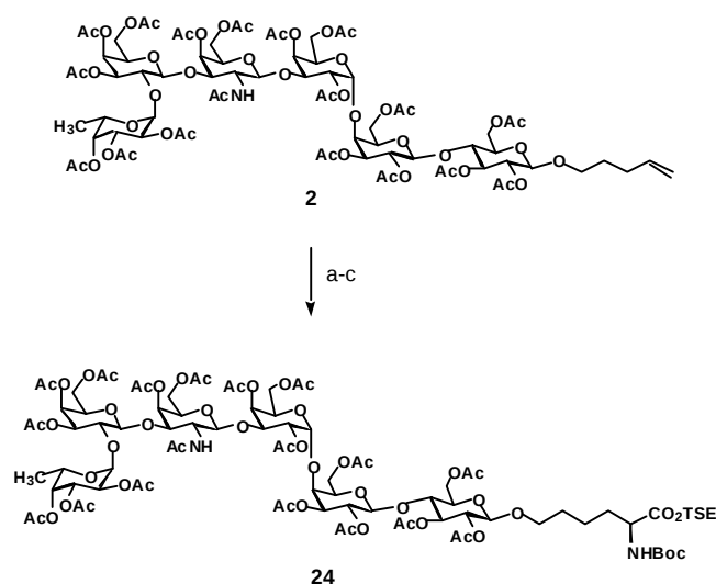
Scheme 5 Synthesis of Globo-H derived glycoamino acid a Key: a) O 3 , MeOH, DCM; Me 2 S; b) TMG, THF, 8d (R = TSE, R' = Boc), –78 °C, 72% 2 steps; c) (S, S)-Et-DuPHOS-Rh + , THF, 50 psi, 98%, dr >20:1.
